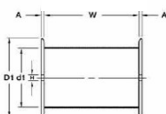
Straight spool
