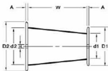
Tapered spool
